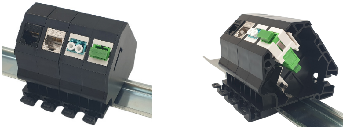
Keystone Modules shown from left to right: Cat6, Cat6a, LC, SC.
